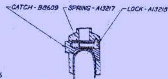
SECTION B-B MAGAZINE LOCKED BY MAGAZINE CATCH
